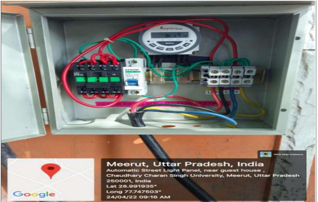
Timer Based Street Light Switches
