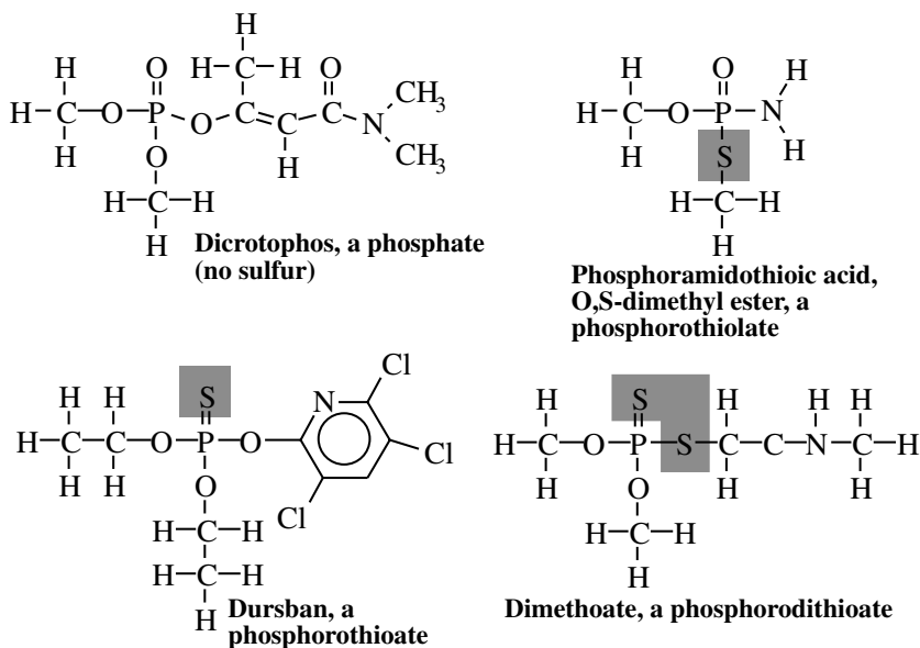
Figure 18.7 Phosphates, phosphorothioate, phosphorothioate, and phosphorodithioate insecticides distinguished by the numbers and orientations of the sulfur atoms around the phosphorus.
