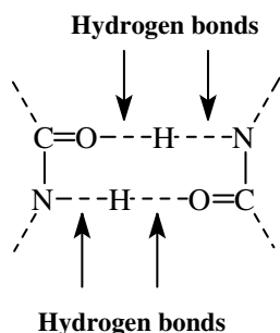
Illustration of hydrogen bonds between N and O atoms in peptide linkages, which constitutes protein secondary structures
