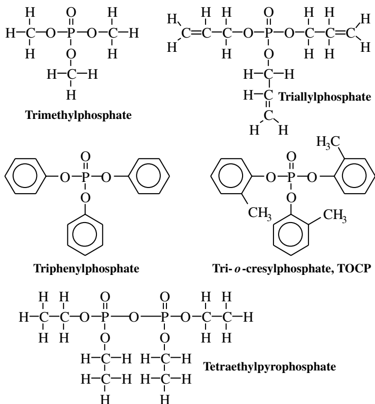
Figure 18.5 Phosphate esters.
