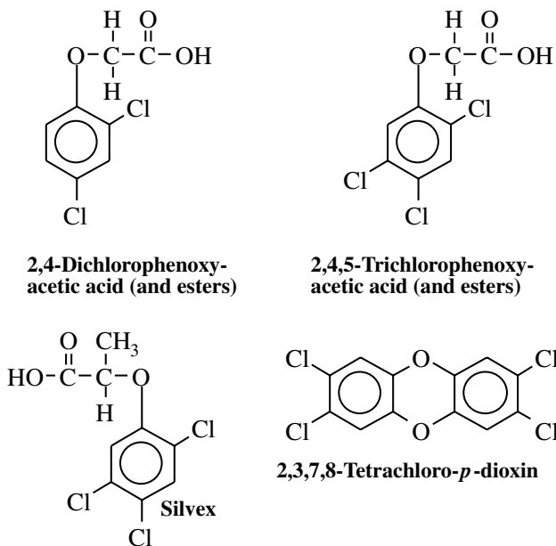
Figure 16.6 Herbicidal chlorophenoxy compounds and TCDD manufacturing by-product.
