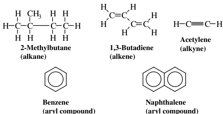
Figure 1.9 Examples of major types of hydrocarbons.
