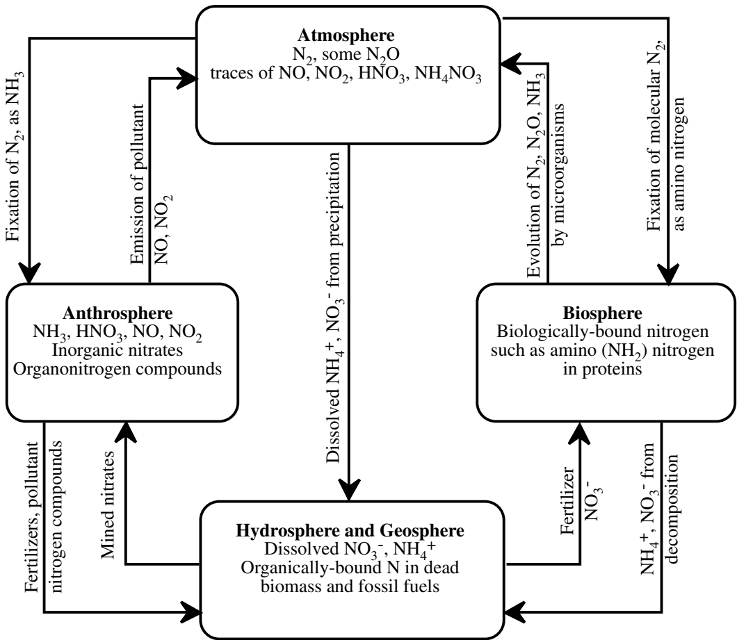
Figure 2.2 The nitrogen cycle.
