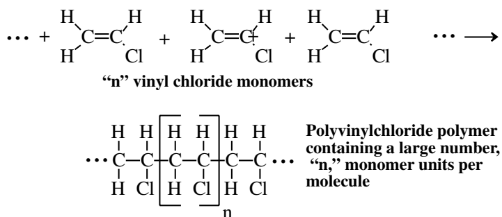
Figure 1.21 Polyvinylchloride polymer.
