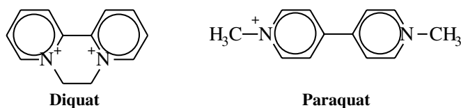
Figure 15.9 The two major bipyridilium herbicides (cation forms).
