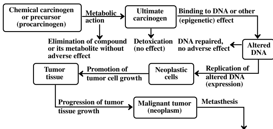
Figure 7.16 Outline of the carcinogenic process.
